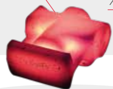
Fluid end / 17-4ph 345kg/760lbs
